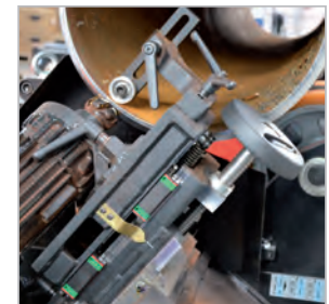
Optional Oval Pipe Tracking Attachment allows out of round pipe beveling
