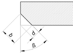
Fig. 1. Bevel dimensions; maximum bevel width depending on the angle
